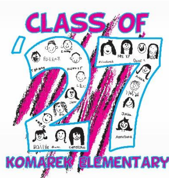
Streaks
