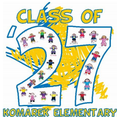
Stars
